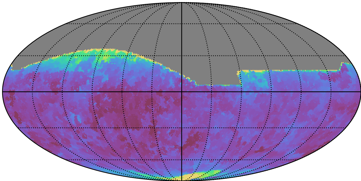
telescope_jerk_v3.5_10yrs All sky r band: Min seeingEff
