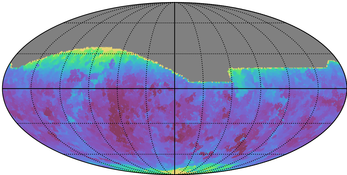
telescope_jerk_v3.5_10yrs All sky i band: Min seeingEff
