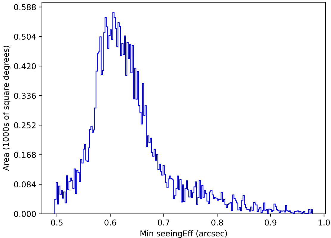
telescope_jerk_v3.5_10yrs All sky i band: Min seeingEff
