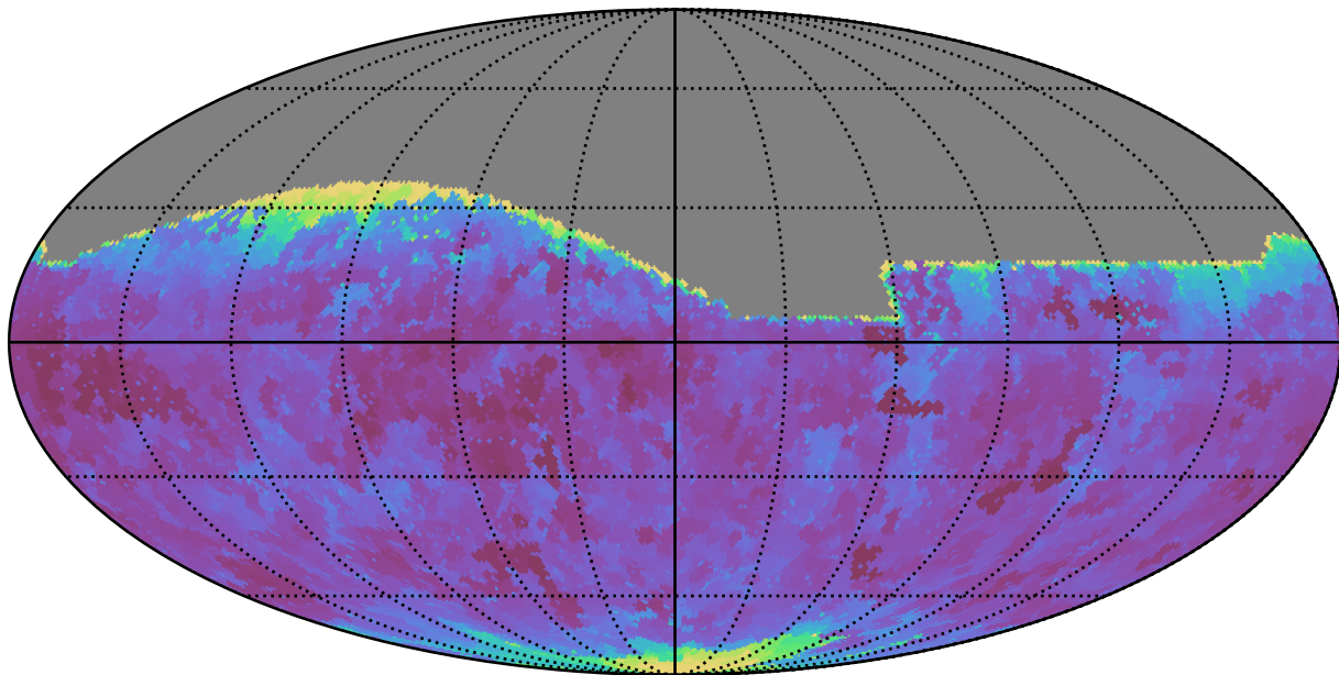
telescope_jerk_v3.5_10yrs All sky g band: Min seeingEff
