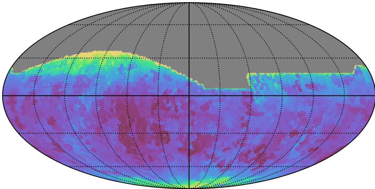
telescope_jerk_v3.5_10yrs All sky all bands: Min seeingEff
