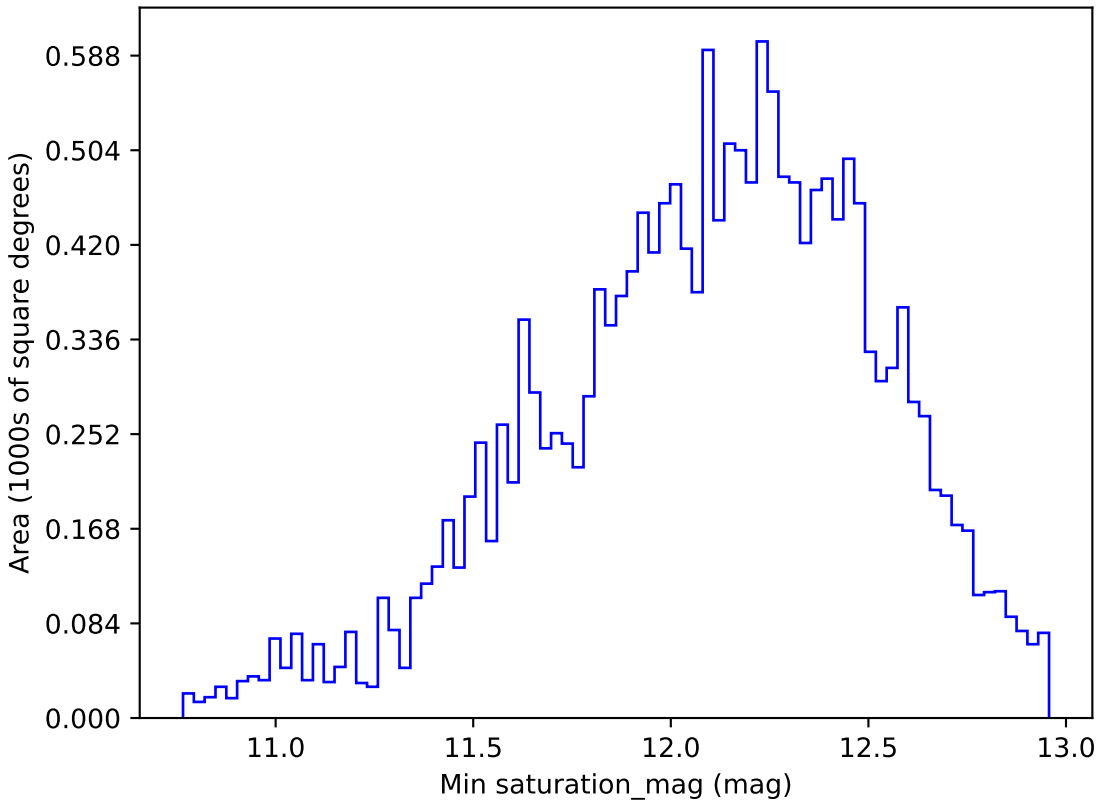
telescope_jerk_v3.5_10yrs WFD z band: Min saturation_mag
