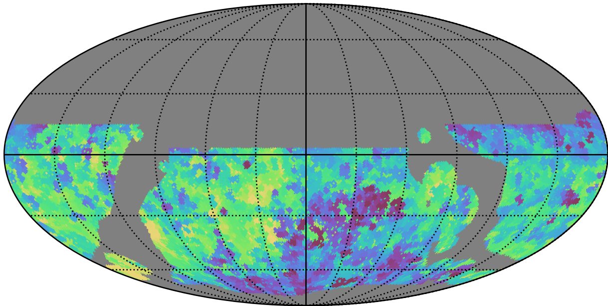
telescope_jerk_v3.5_10yrs WFD u band: Min saturation_mag
