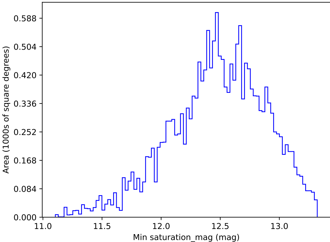
telescope_jerk_v3.5_10yrs WFD r band: Min saturation_mag
