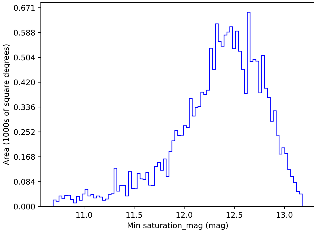
telescope_jerk_v3.5_10yrs WFD i band: Min saturation_mag
