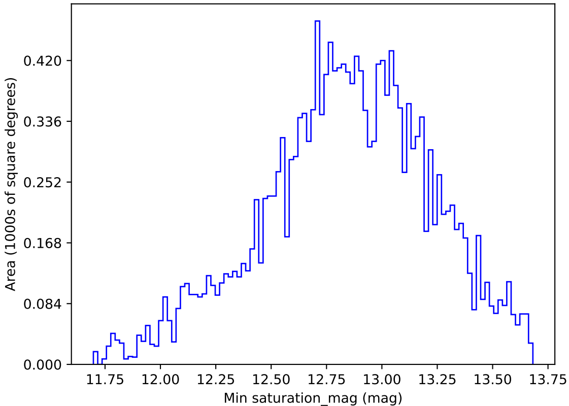
telescope_jerk_v3.5_10yrs WFD g band: Min saturation_mag
