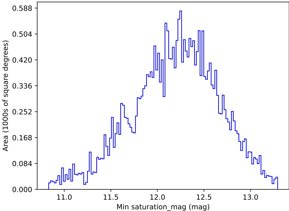
telescope_jerk_v3.5_10yrs All sky z band: Min saturation_mag
