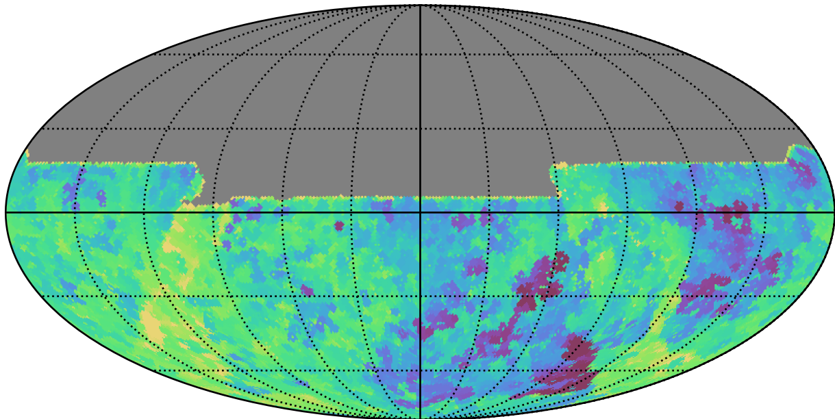
telescope_jerk_v3.5_10yrs All sky y band: Min saturation_mag
