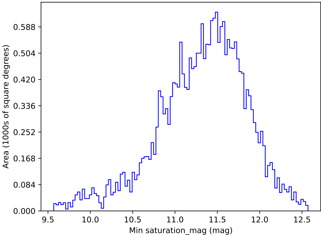
telescope_jerk_v3.5_10yrs All sky y band: Min saturation_mag
