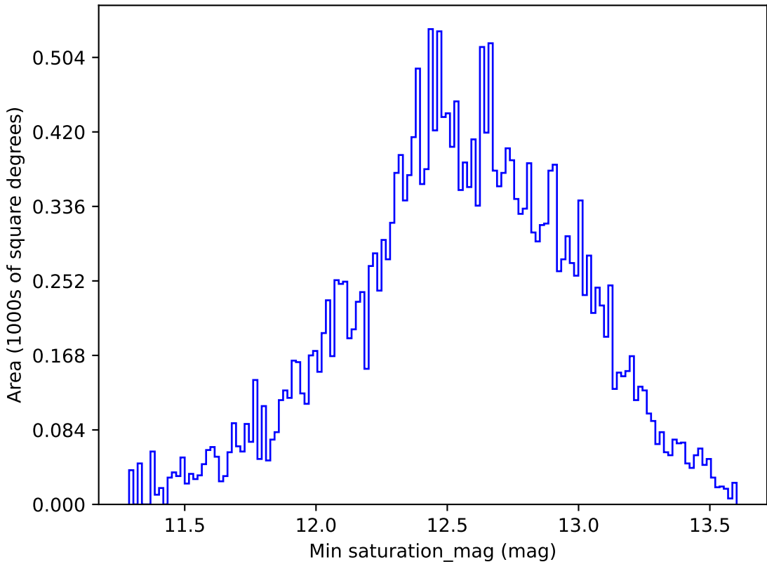
telescope_jerk_v3.5_10yrs All sky r band: Min saturation_mag
