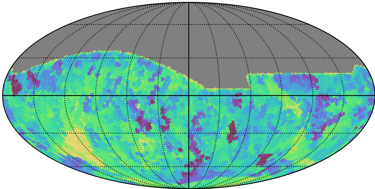
telescope_jerk_v3.5_10yrs All sky i band: Min saturation_mag
