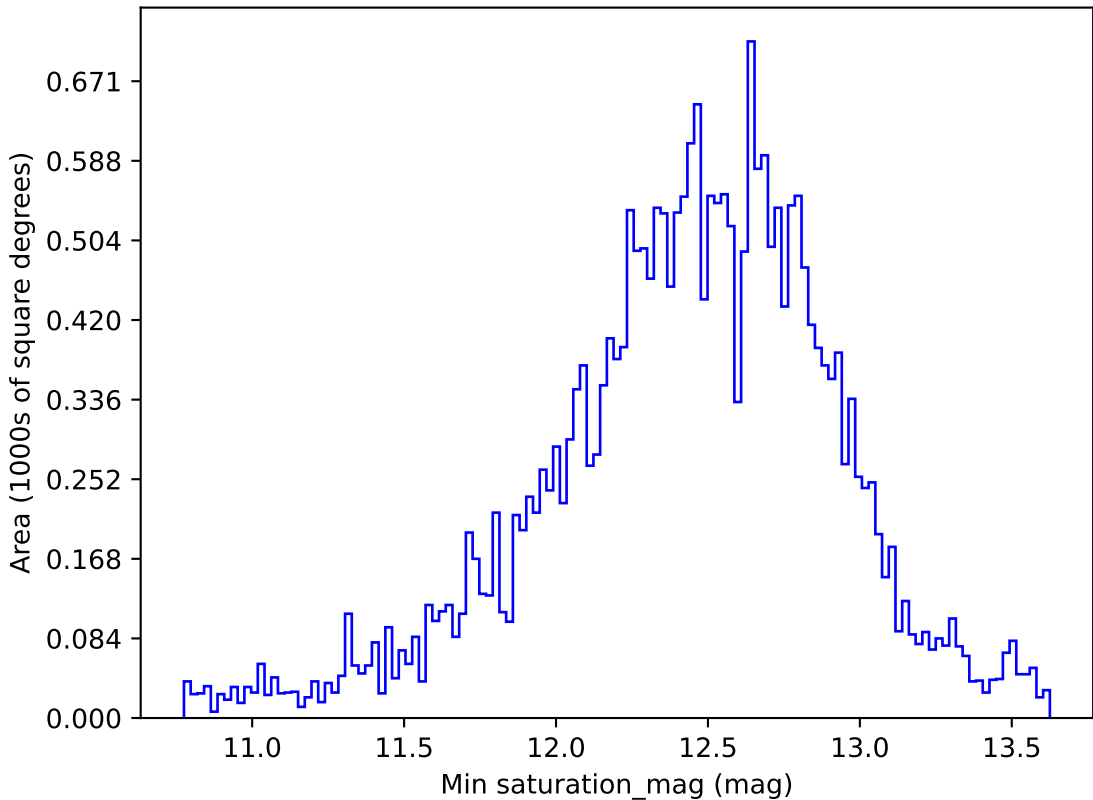
telescope_jerk_v3.5_10yrs All sky i band: Min saturation_mag
