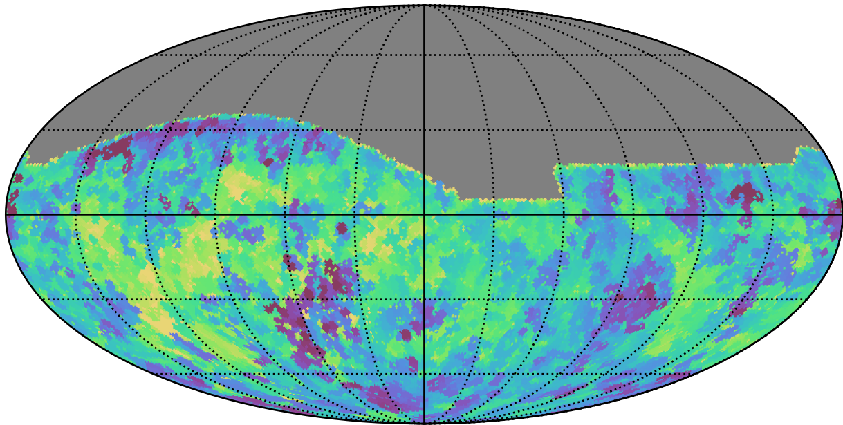
telescope_jerk_v3.5_10yrs All sky g band: Min saturation_mag
