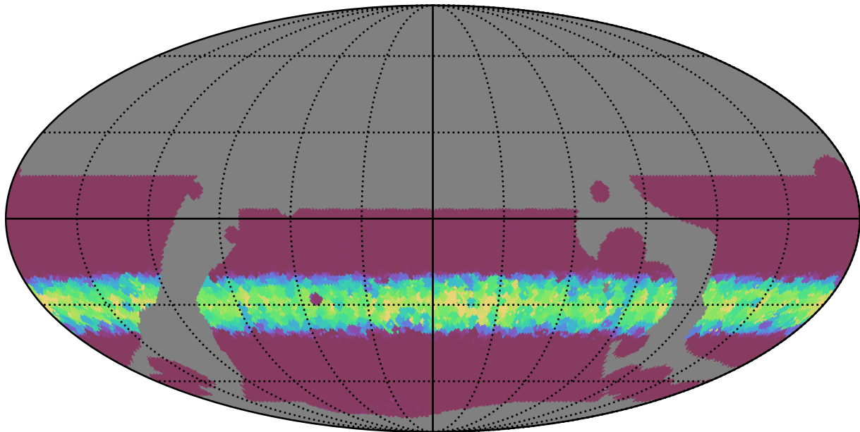
telescope_jerk_v3.5_10yrs WFD z band: Min normairmass
