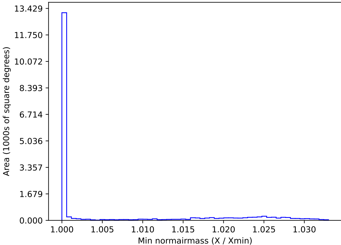
telescope_jerk_v3.5_10yrs WFD z band: Min normairmass
