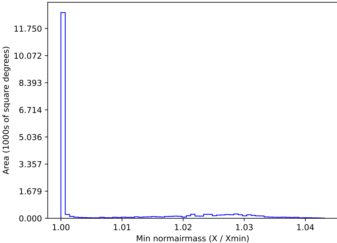
telescope_jerk_v3.5_10yrs WFD y band: Min normairmass
