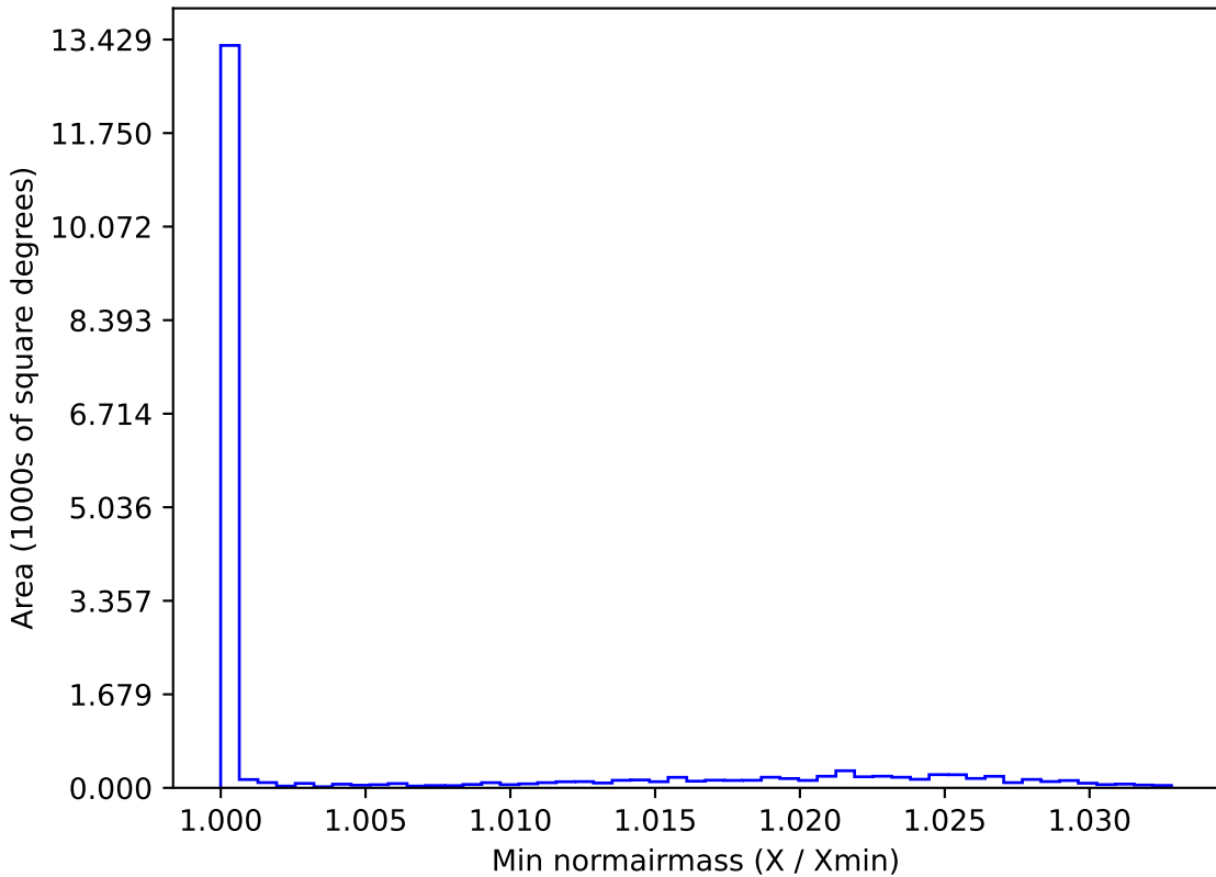
telescope_jerk_v3.5_10yrs WFD r band: Min normairmass
