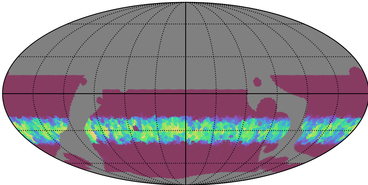
telescope_jerk_v3.5_10yrs WFD g band: Min normairmass
