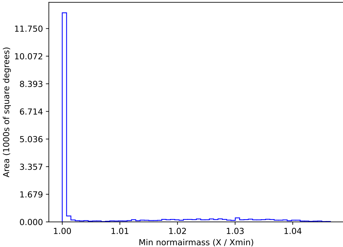
telescope_jerk_v3.5_10yrs WFD g band: Min normairmass
