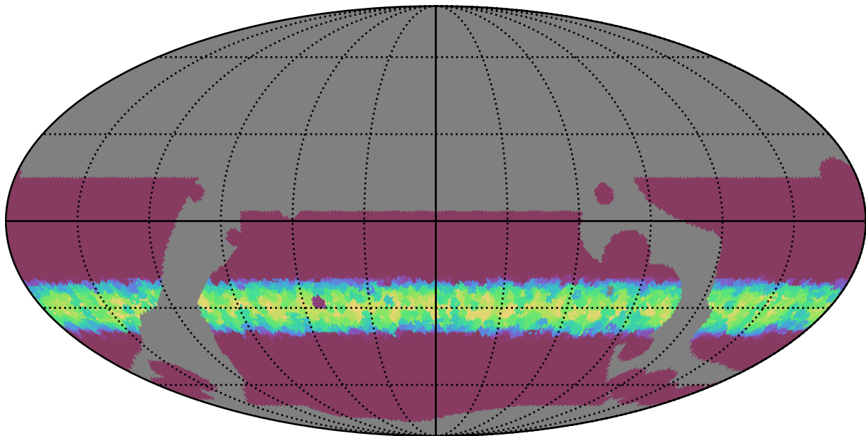
telescope_jerk_v3.5_10yrs WFD all bands: Min normairmass
