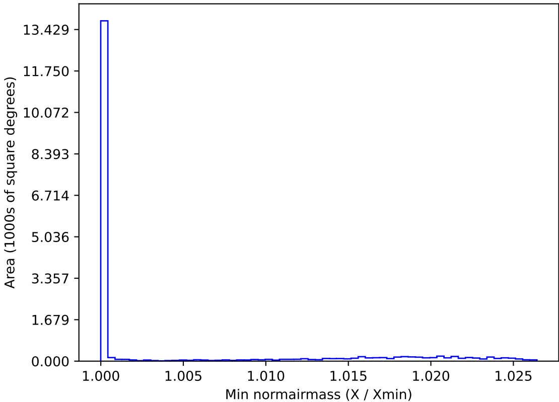
telescope_jerk_v3.5_10yrs WFD all bands: Min normairmass
