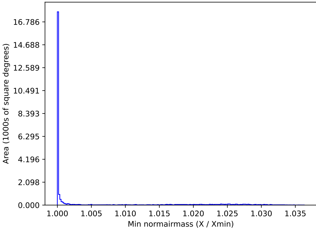
telescope_jerk_v3.5_10yrs All sky z band: Min normairmass
