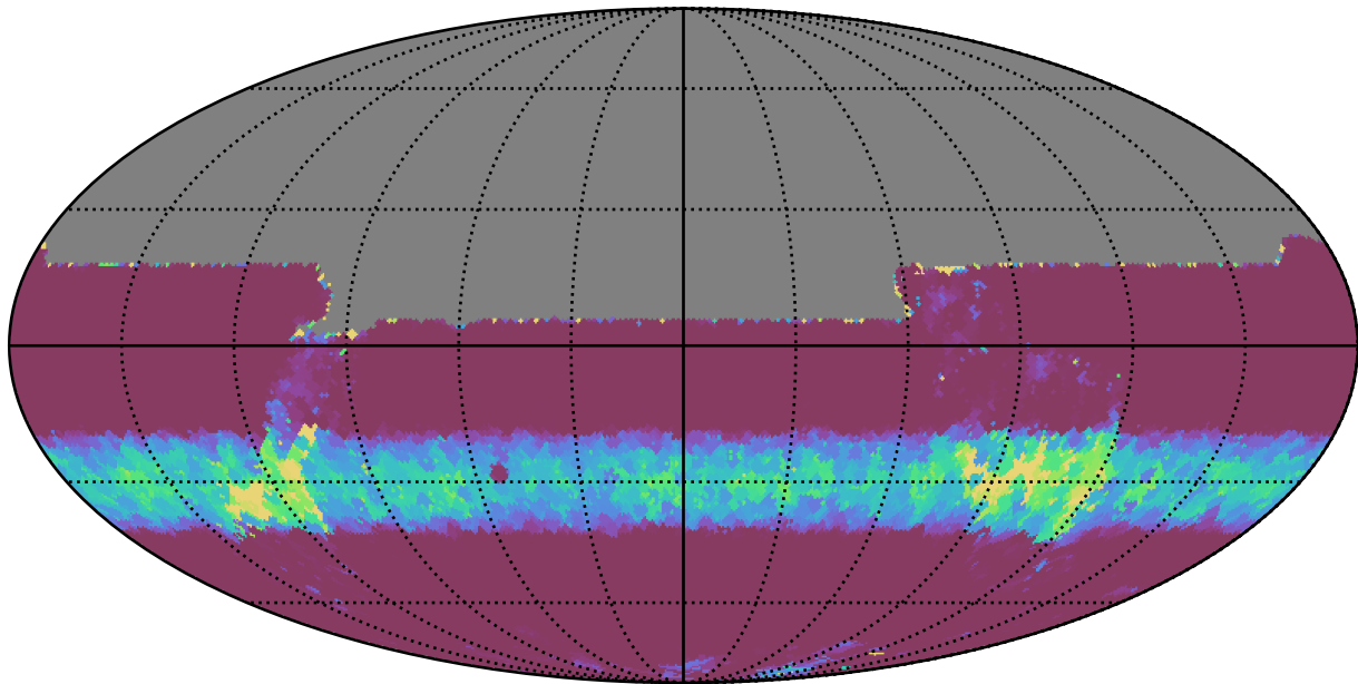
telescope_jerk_v3.5_10yrs All sky y band: Min normairmass
