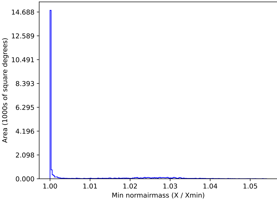
telescope_jerk_v3.5_10yrs All sky y band: Min normairmass
