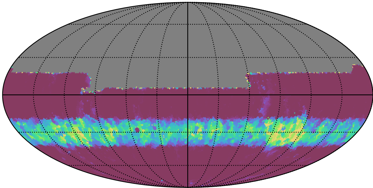
telescope_jerk_v3.5_10yrs All sky u band: Min normairmass
