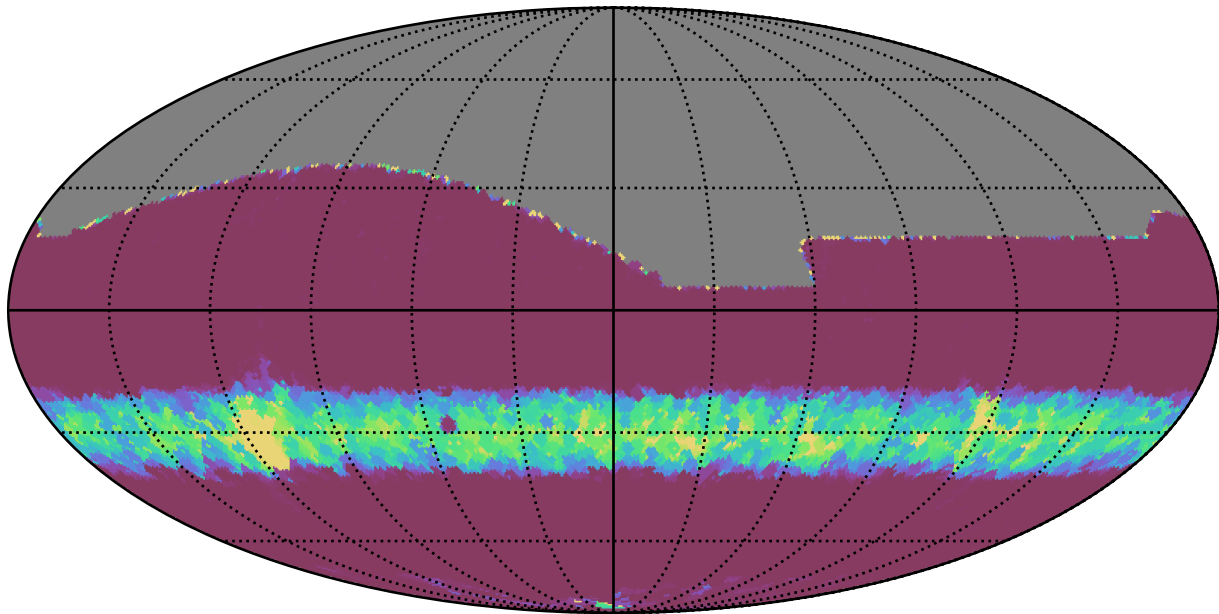
telescope_jerk_v3.5_10yrs All sky r band: Min normairmass
