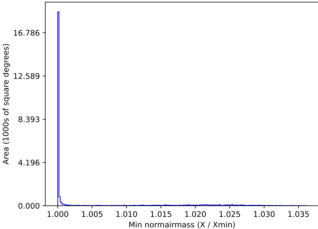
telescope_jerk_v3.5_10yrs All sky r band: Min normairmass
