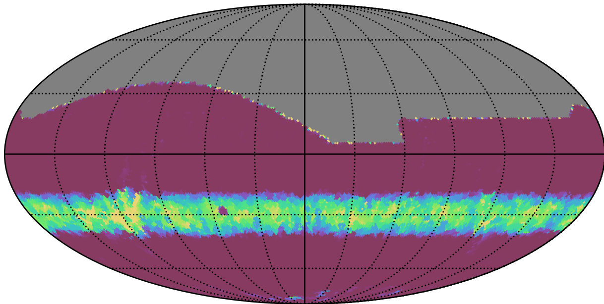
telescope_jerk_v3.5_10yrs All sky i band: Min normairmass
