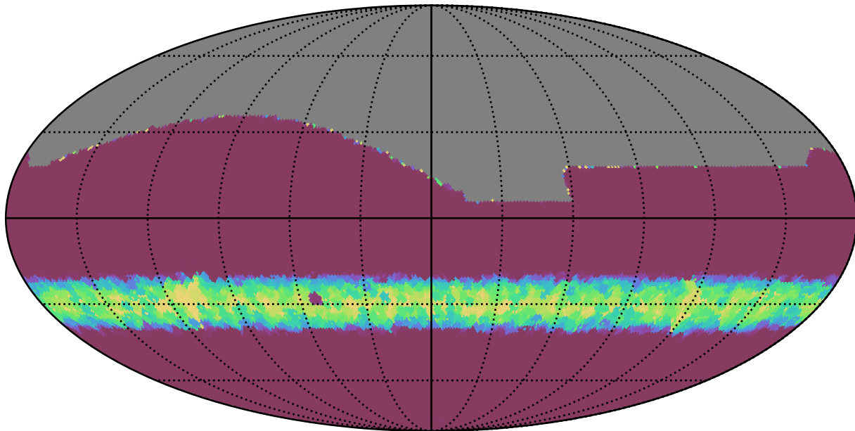
telescope_jerk_v3.5_10yrs All sky all bands: Min normairmass
