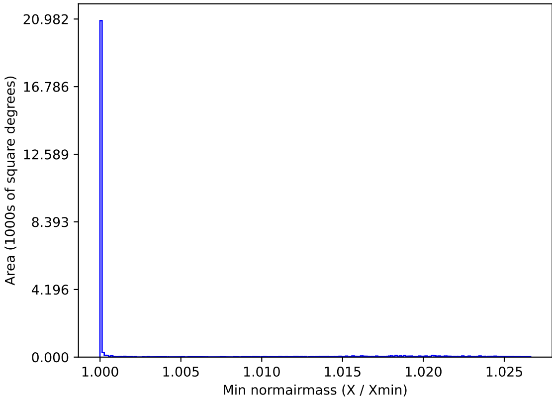
telescope_jerk_v3.5_10yrs All sky all bands: Min normairmass
