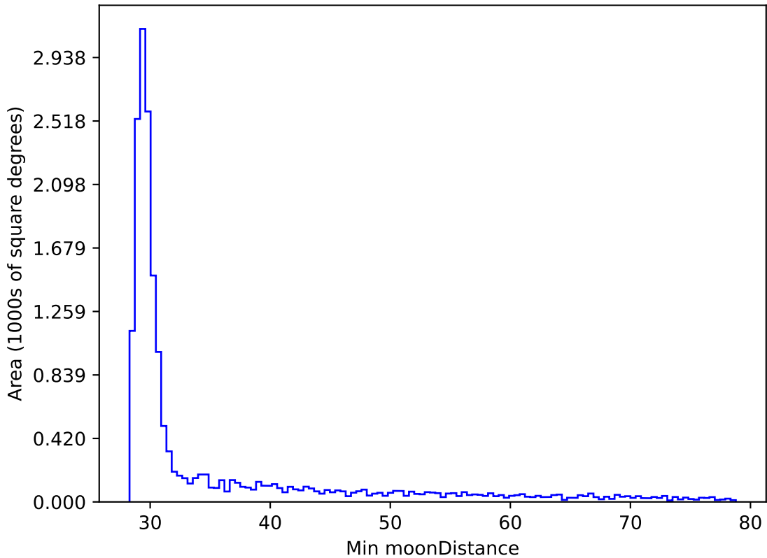
telescope_jerk_v3.5_10yrs WFD y band: Min moonDistance
