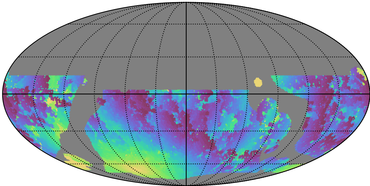
telescope_jerk_v3.5_10yrs WFD u band: Min moonDistance
