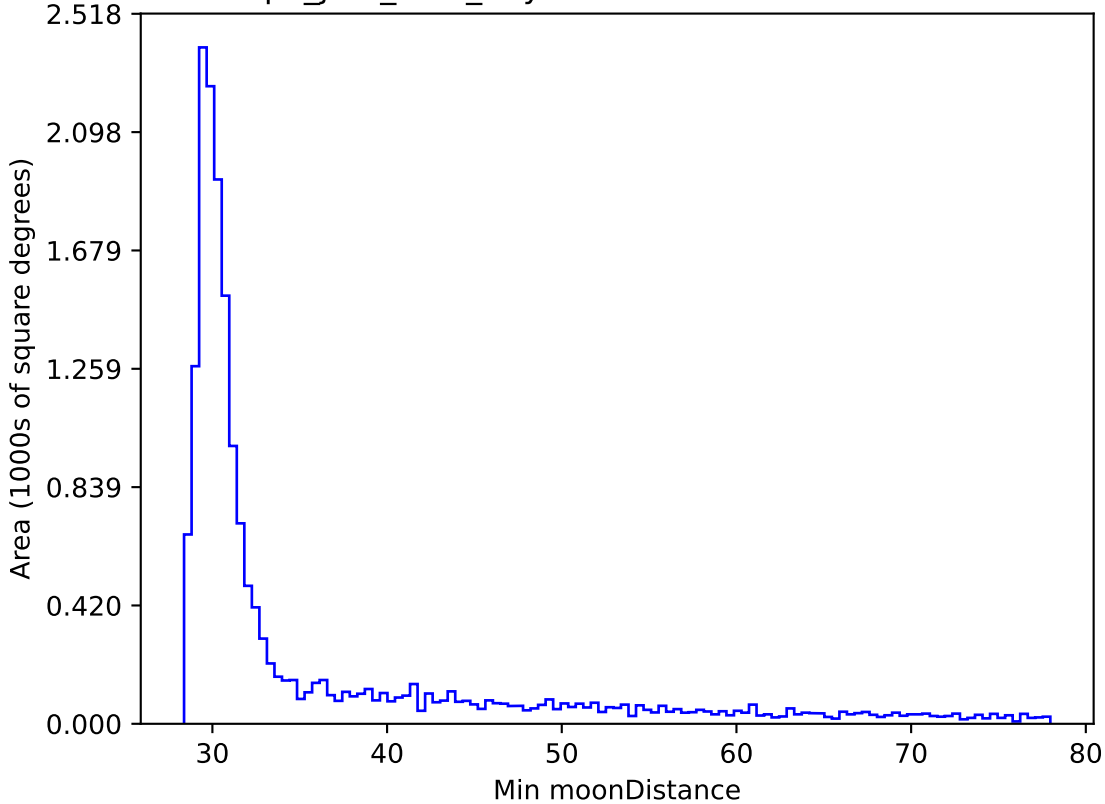
telescope_jerk_v3.5_10yrs WFD i band: Min moonDistance
