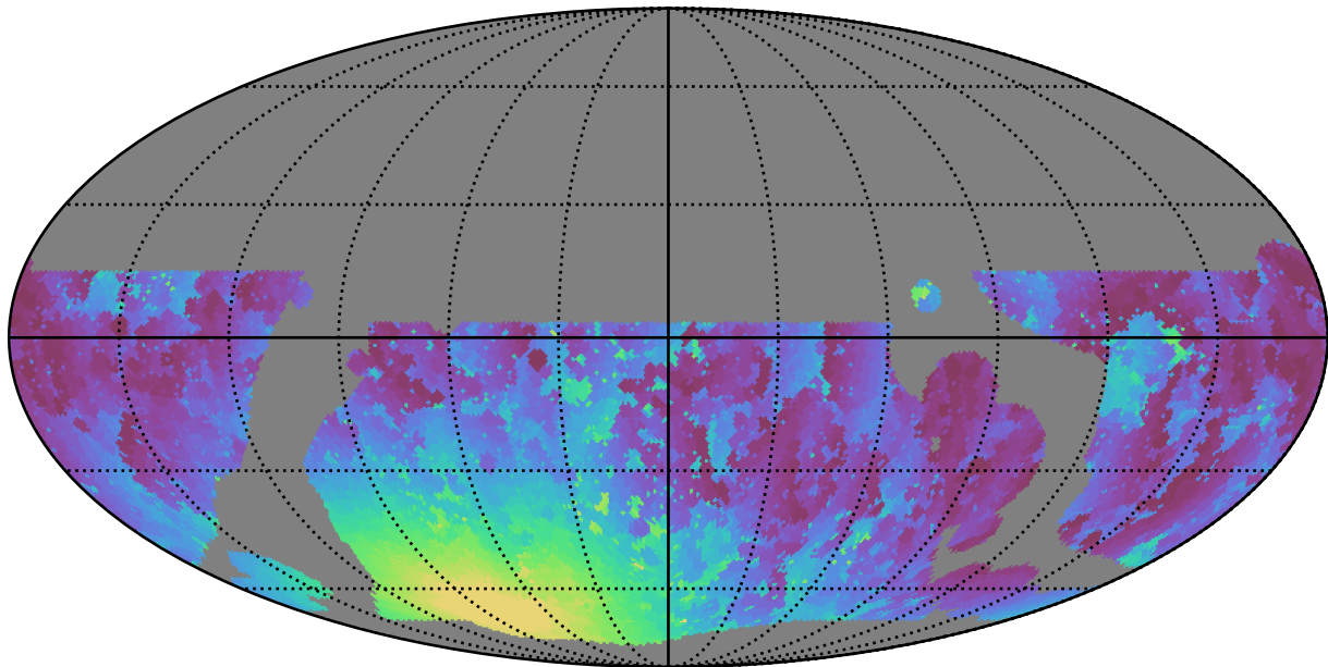
telescope_jerk_v3.5_10yrs WFD g band: Min moonDistance
