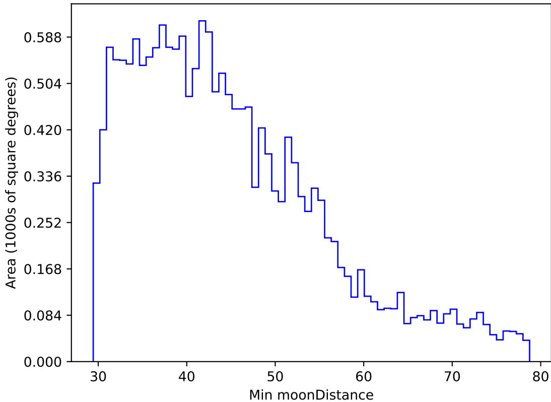
telescope_jerk_v3.5_10yrs WFD g band: Min moonDistance
