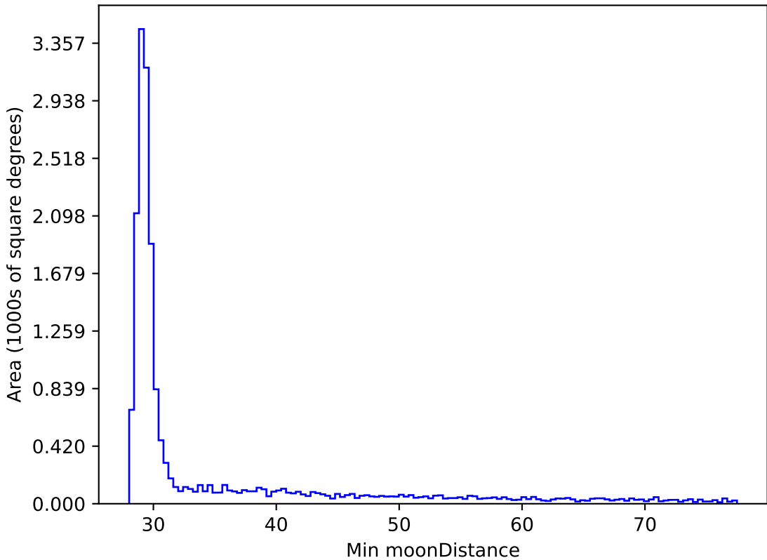
telescope_jerk_v3.5_10yrs WFD all bands: Min moonDistance
