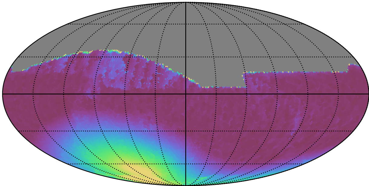
telescope_jerk_v3.5_10yrs All sky z band: Min moonDistance
