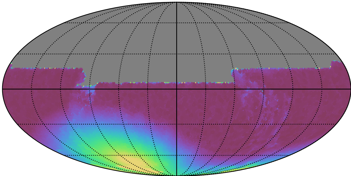
telescope_jerk_v3.5_10yrs All sky y band: Min moonDistance
