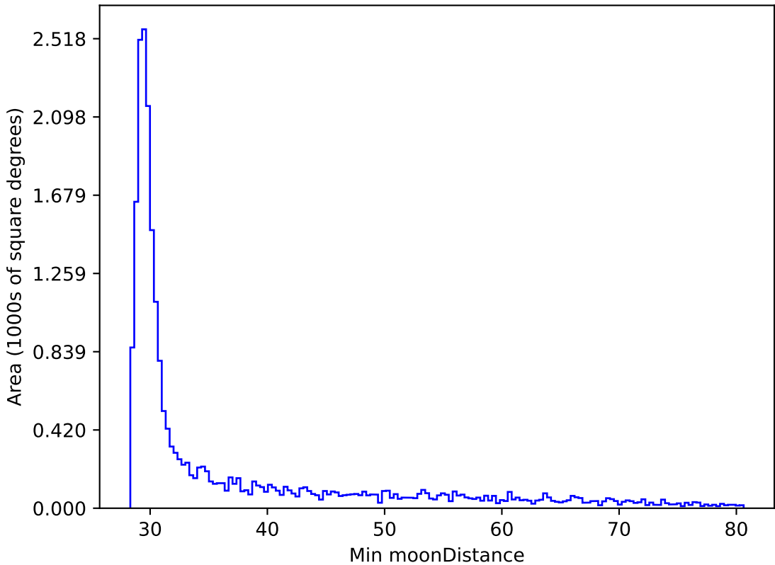
telescope_jerk_v3.5_10yrs All sky y band: Min moonDistance
