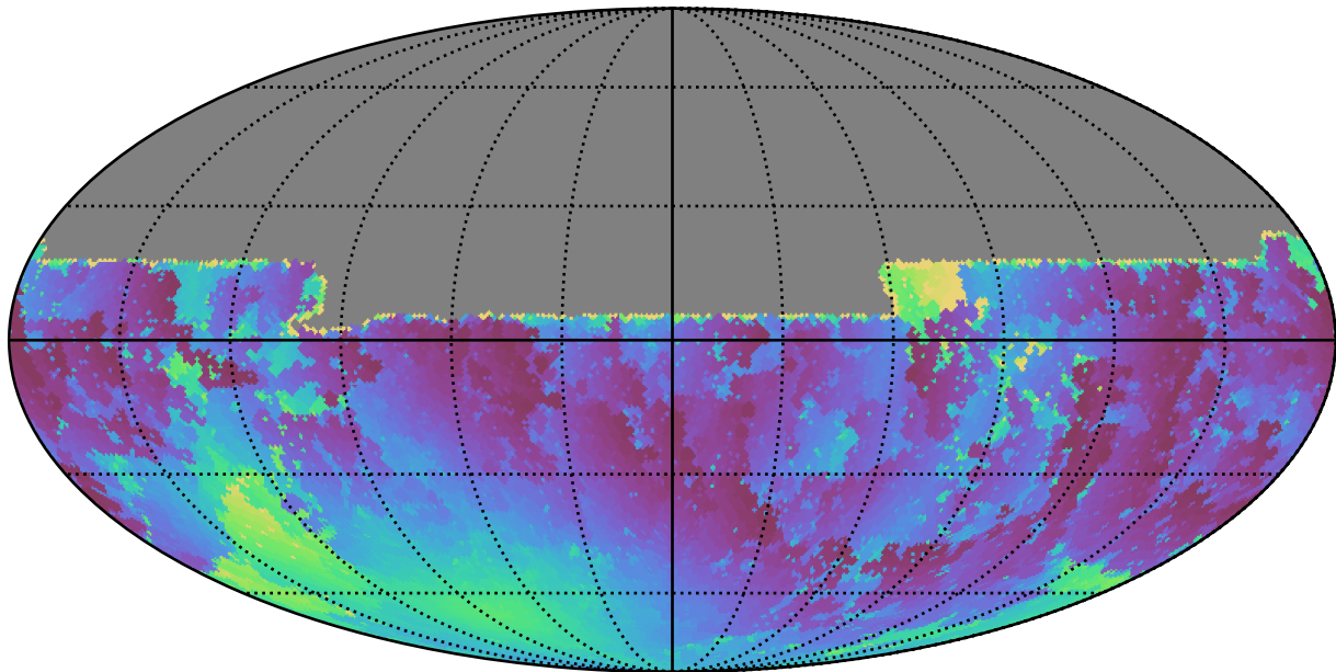
telescope_jerk_v3.5_10yrs All sky u band: Min moonDistance
