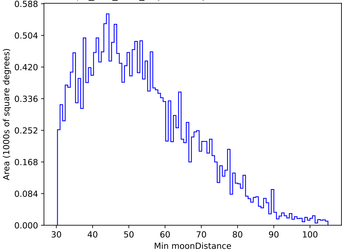
telescope_jerk_v3.5_10yrs All sky u band: Min moonDistance
