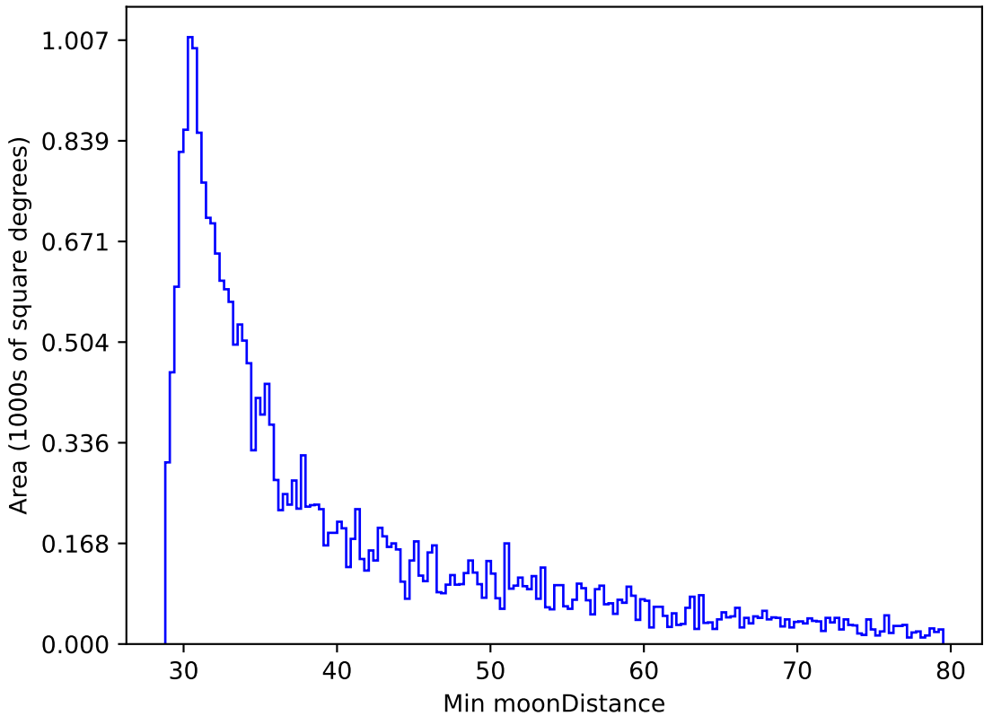
telescope_jerk_v3.5_10yrs All sky r band: Min moonDistance
