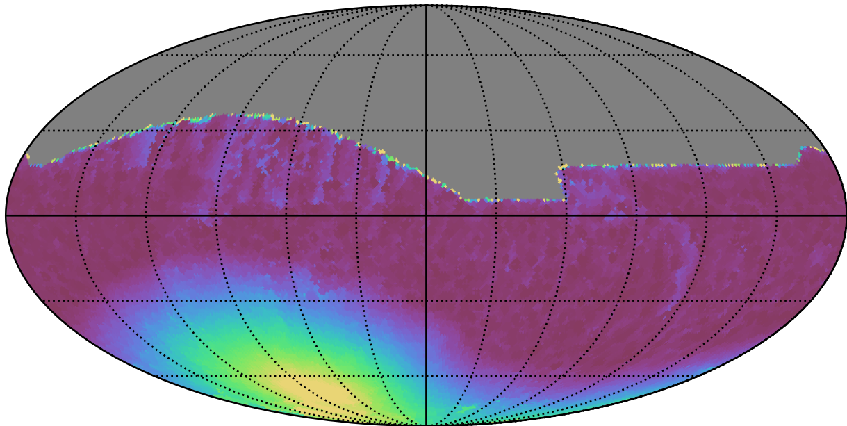
telescope_jerk_v3.5_10yrs All sky i band: Min moonDistance
