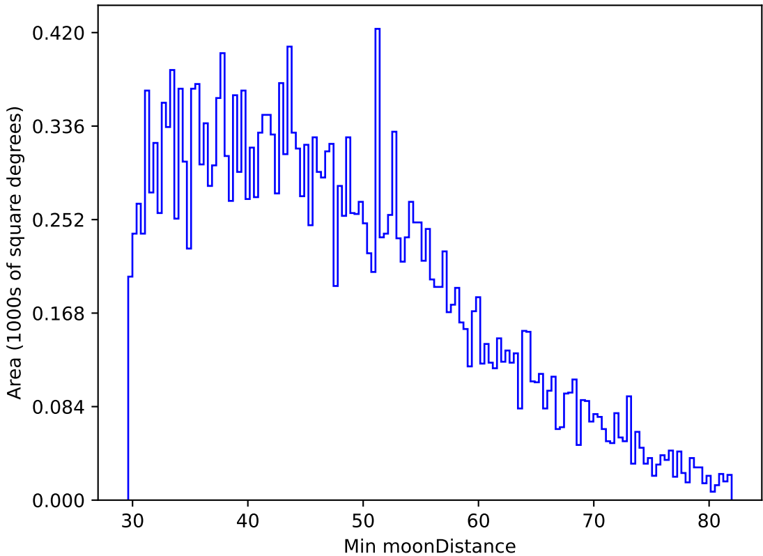
telescope_jerk_v3.5_10yrs All sky g band: Min moonDistance
