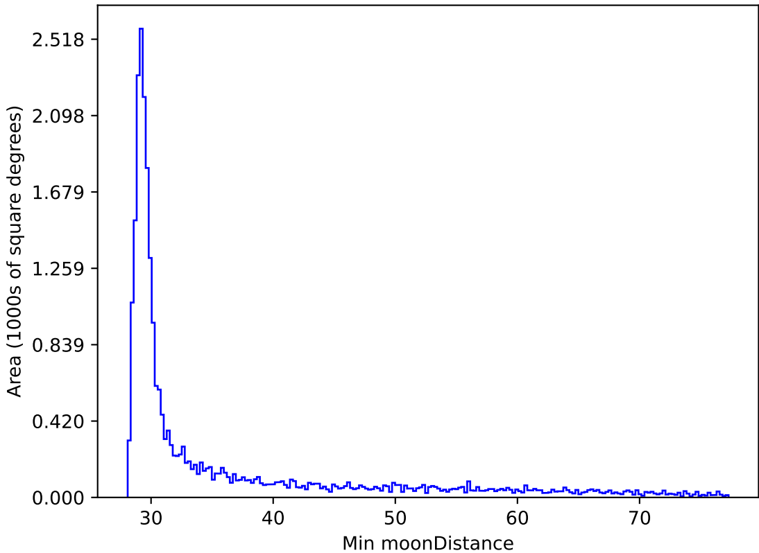
telescope_jerk_v3.5_10yrs All sky all bands: Min moonDistance
