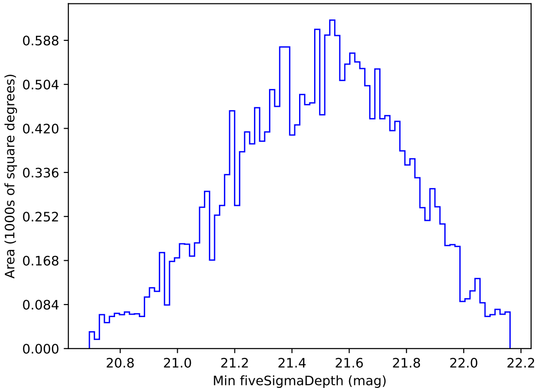
telescope_jerk_v3.5_10yrs Yr 1 y band: Min fiveSigmaDepth
